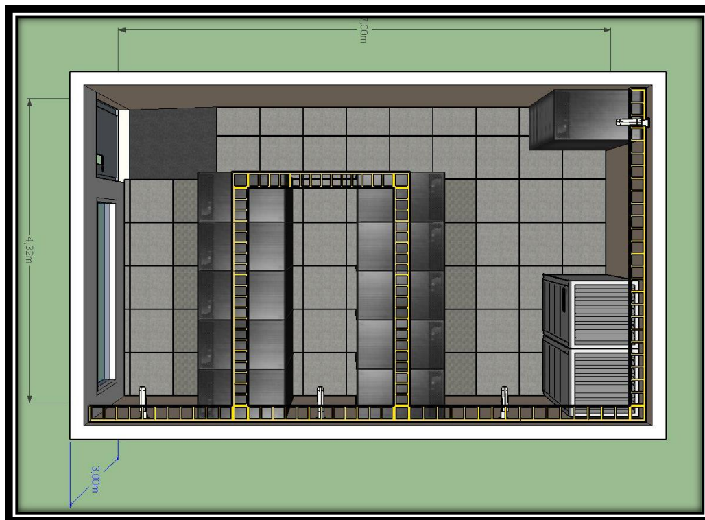
Gambar 5. Layout Datacenter UIN Raden Fatah Palembang
